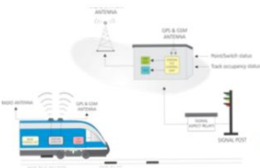
Train Collision Avoidance System
